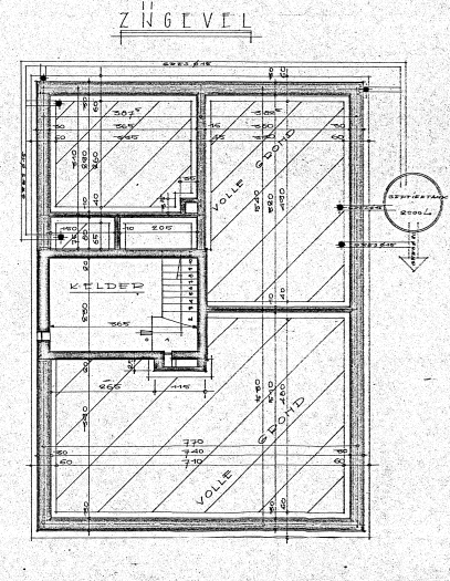
FUNDERINGEN
