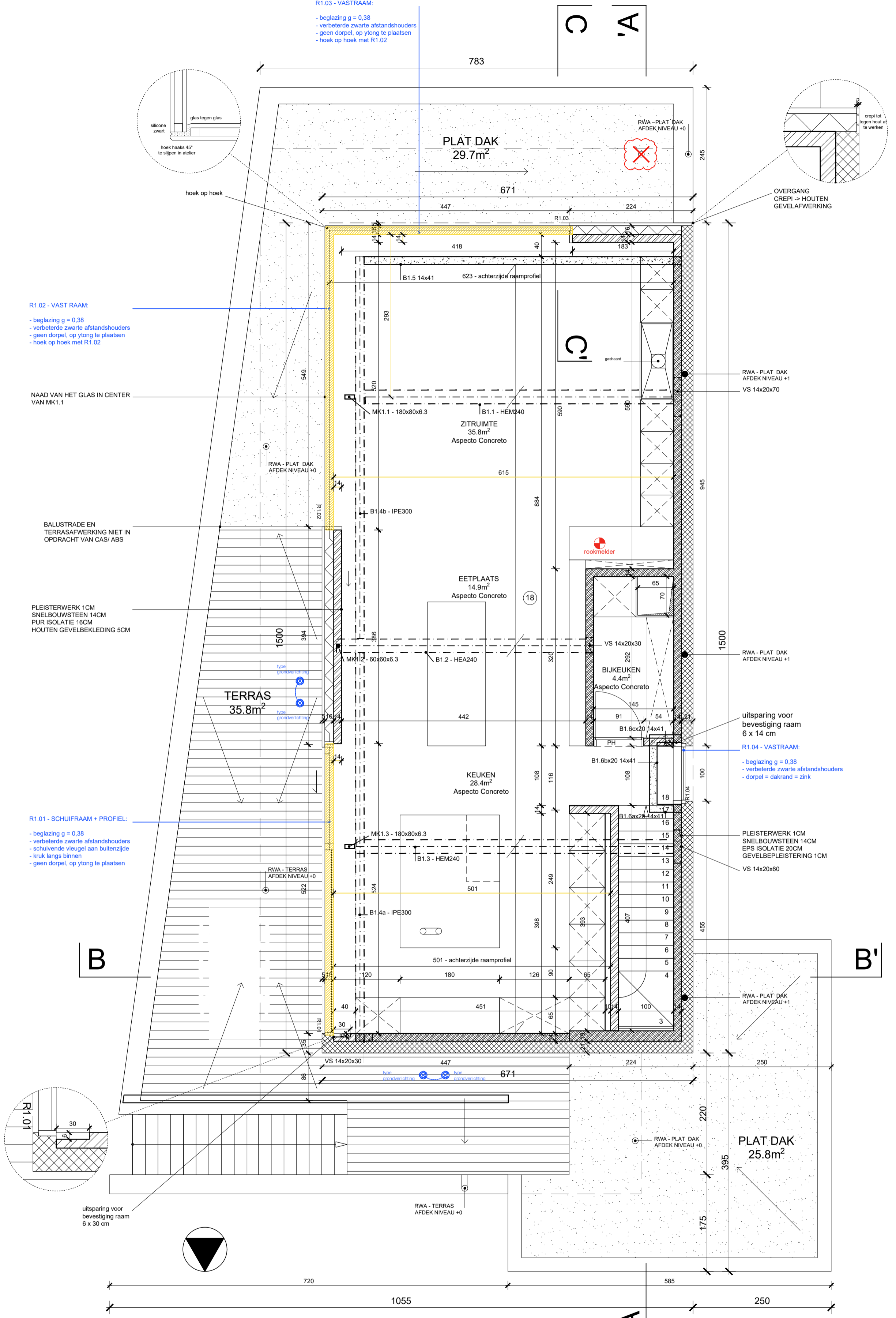
PLAN NIVEAU +1 WONING - BRUTO OPP: 100.6m 2
