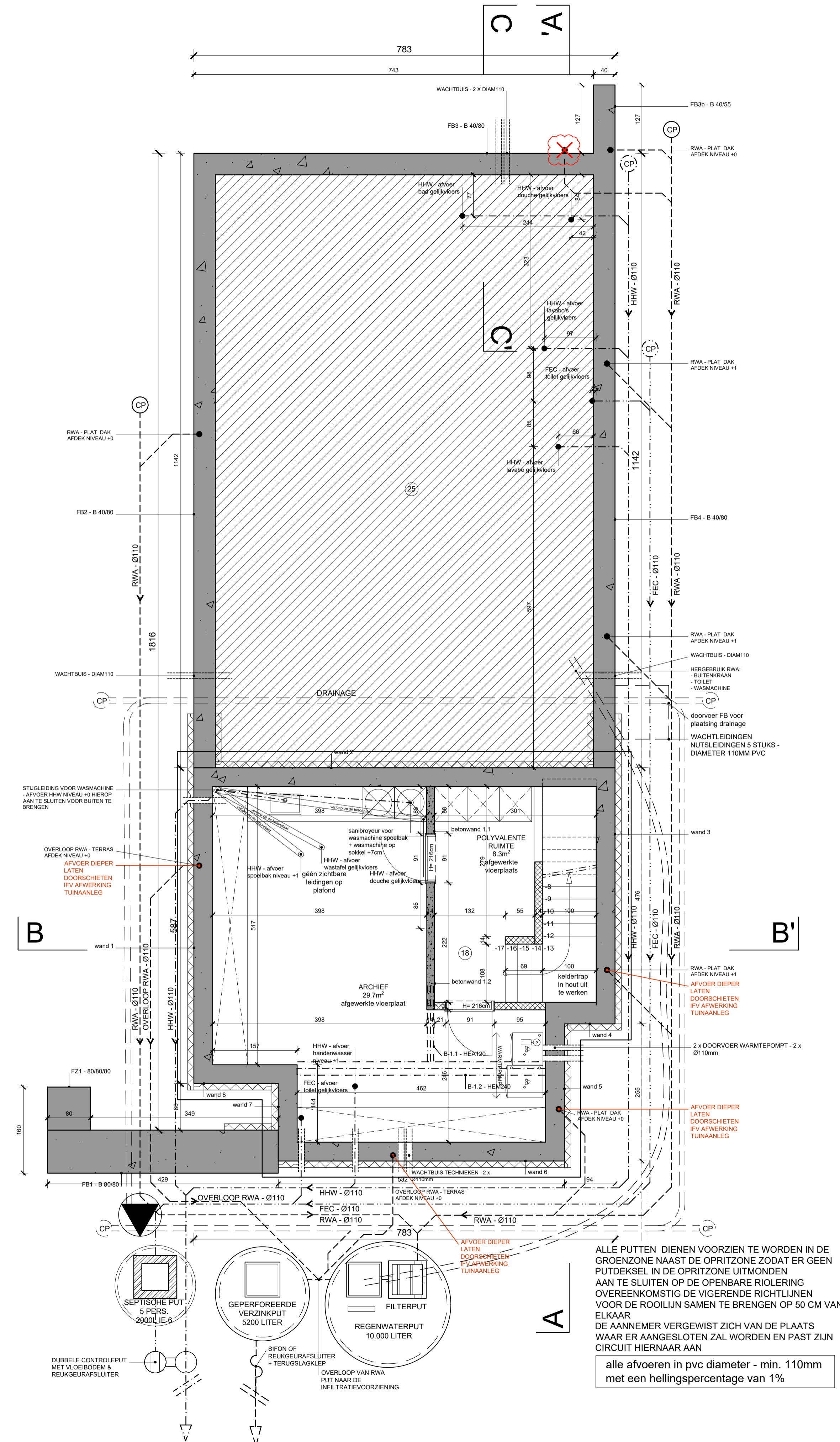
PLAN KELDER- FUNDERING- EN RIOLERING WONING - BRUTO OPP: 52.6m 2
