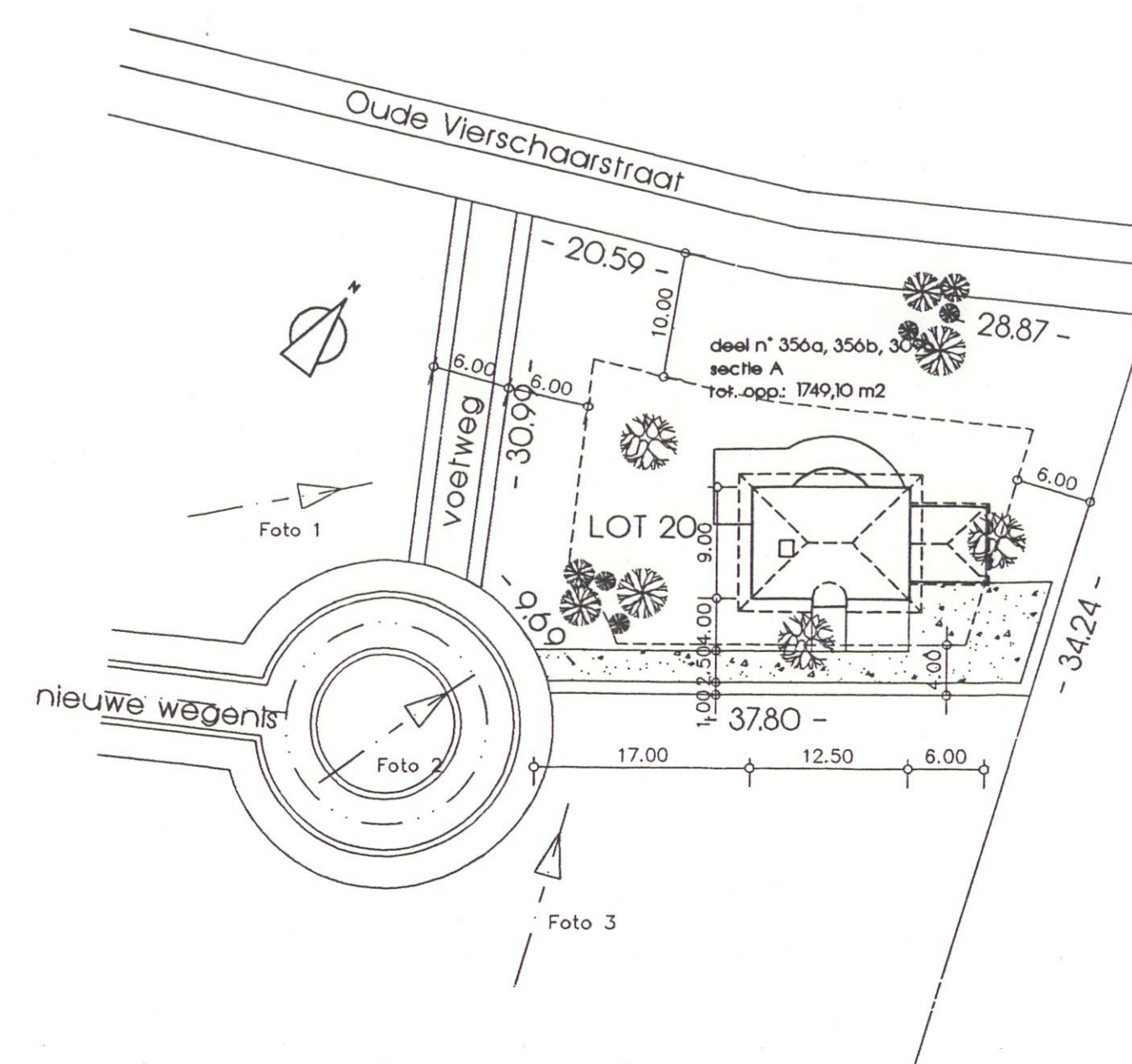
INPLANTINGSPLAN 1/500
