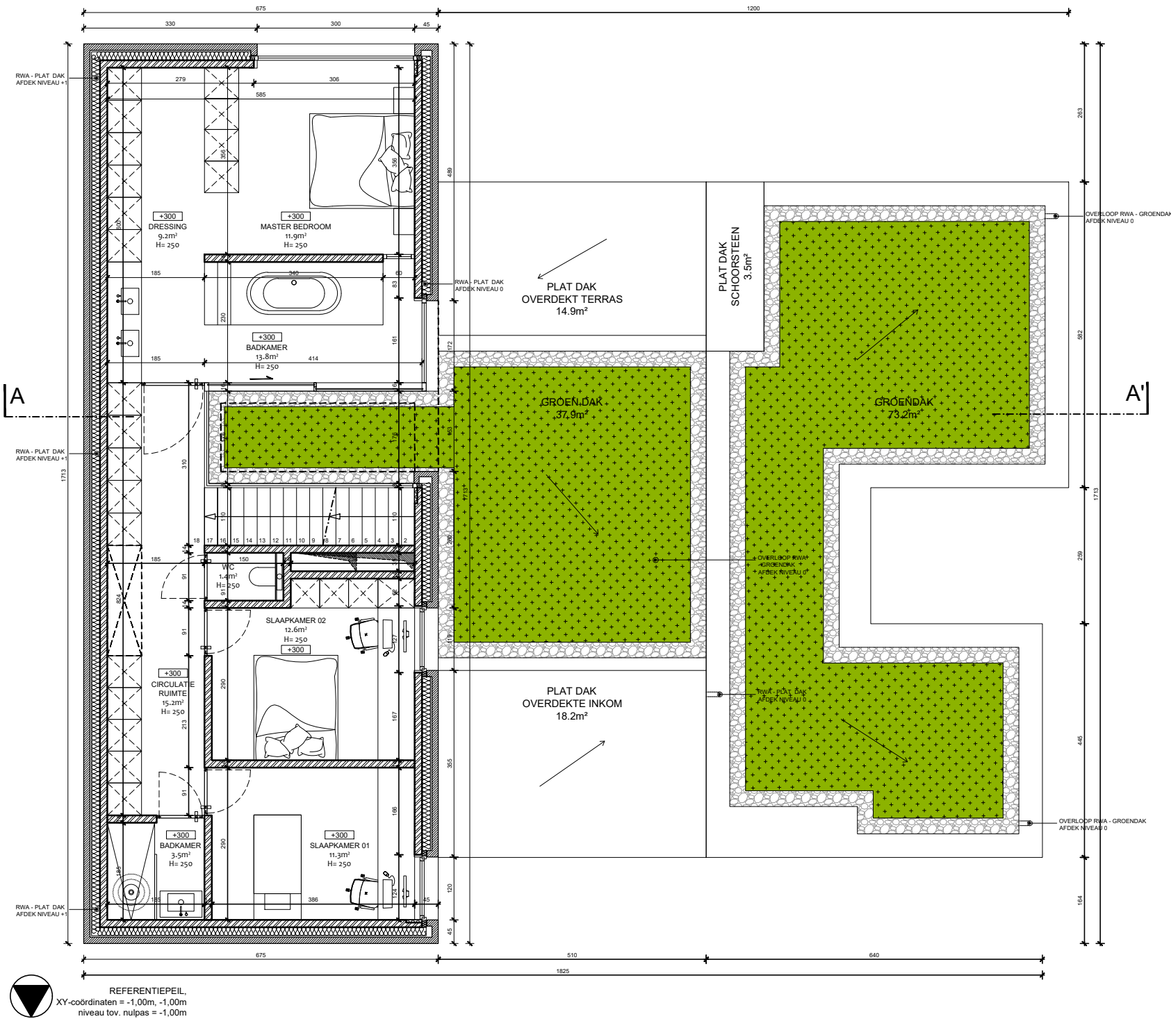
PLAN NIVEAU +1 WONING - versie A - BRUTO OPP: 107.9m²
